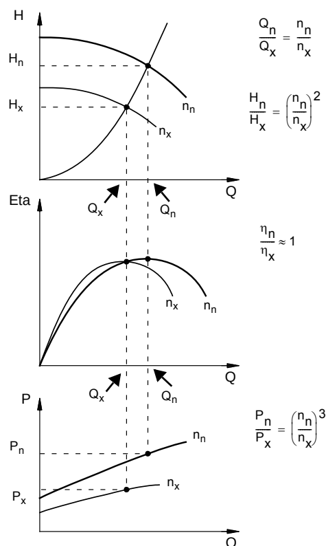
Fig. 84 Equations affines
